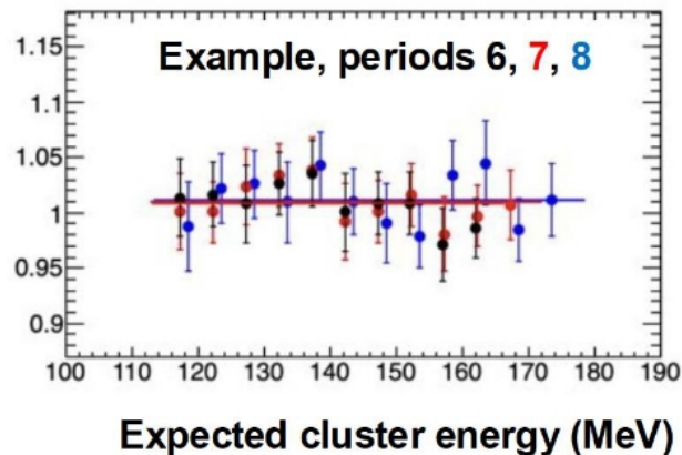
Efficiency Data/MC
