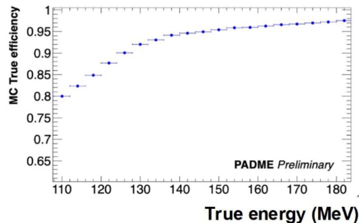
MC True efficiency vs Expected cluster energy (MeV)
